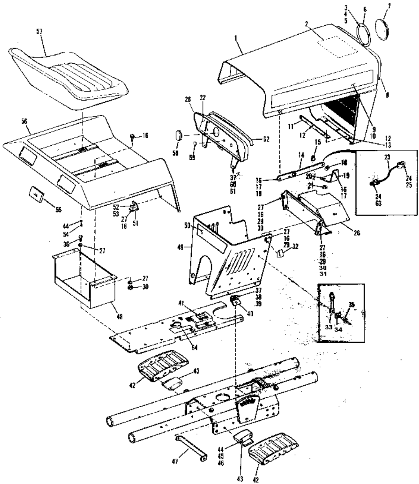
TRIM ASSEMBLY
