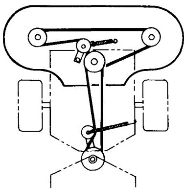
FRAME STEER MODEL 15550
