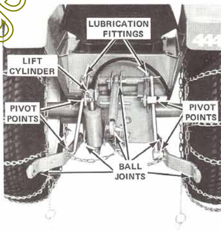
FIGURE 4 Lubrication Points
