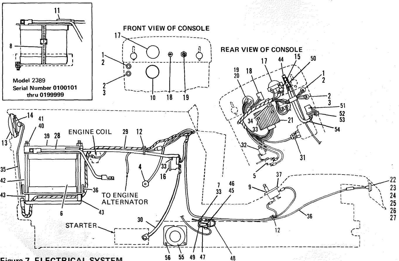
Figure 7 ELECTRICAL SYSTEM
