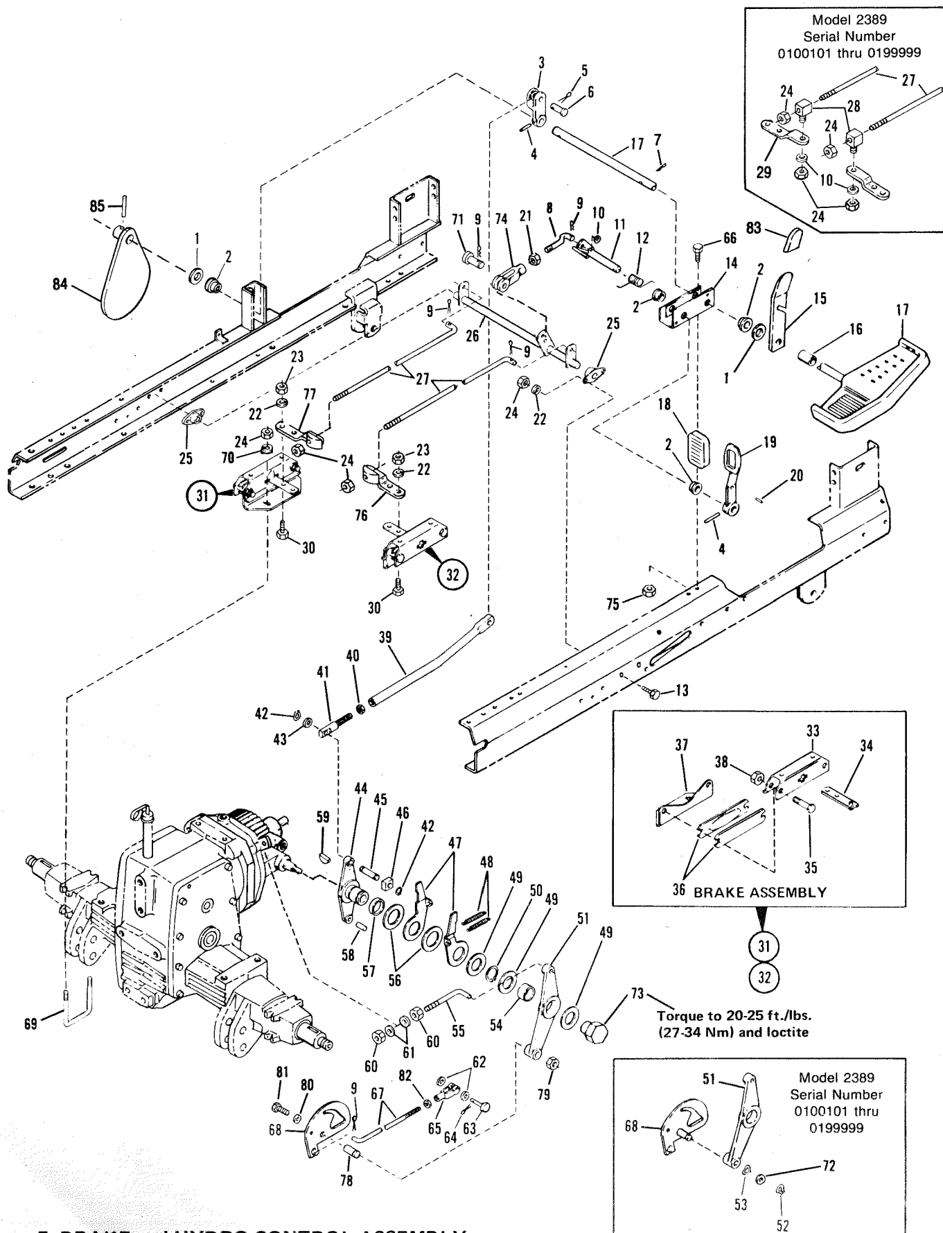
Figure 5 BRAKE and HYDRO CONTROL ASSEMBLY
