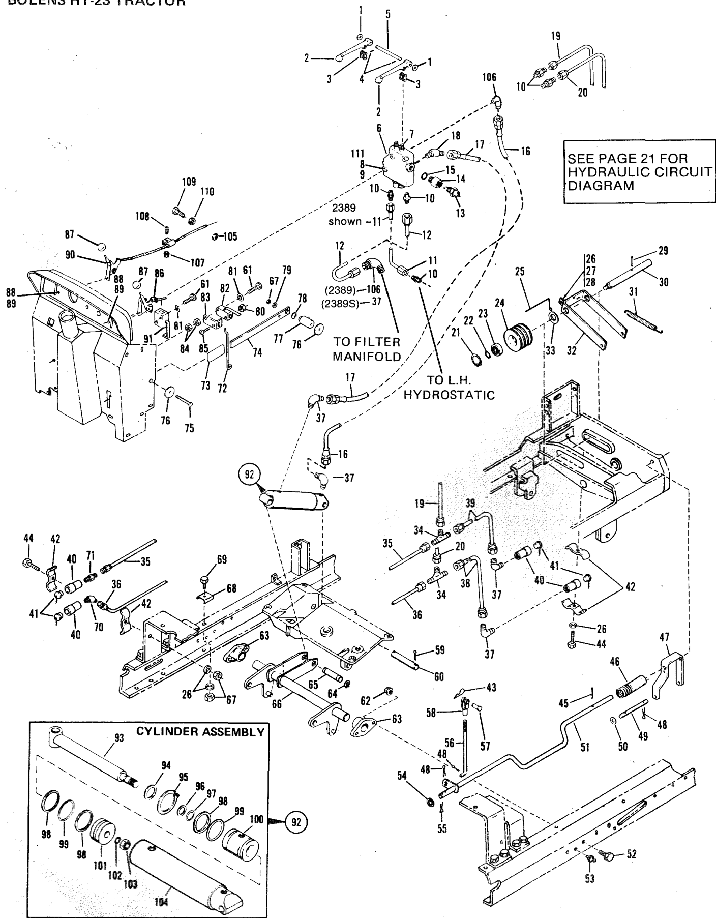
Figure 4 HAND CONTROLS and LIFT ASSEMBLY
