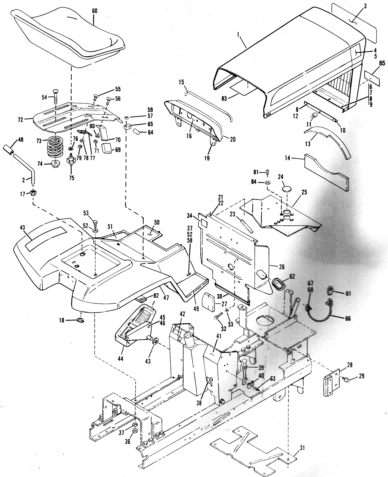
Figure 1 TRIM ASSEMBLY
